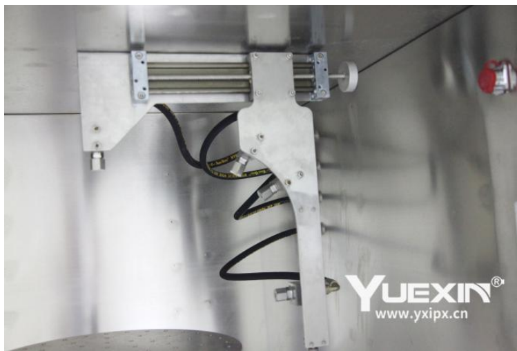
nozzle
